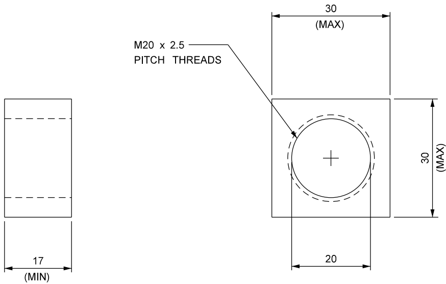
SIDE VIEW 1:1
