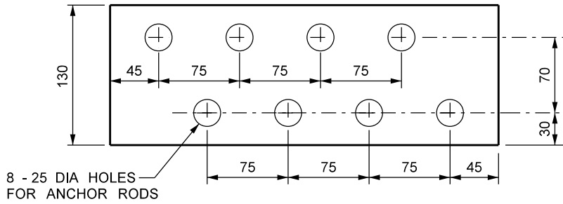
PLAN VIEW 1:5
