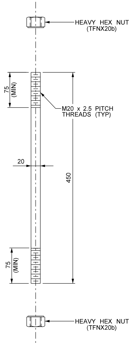
ELEVATION VIEW 1:5
